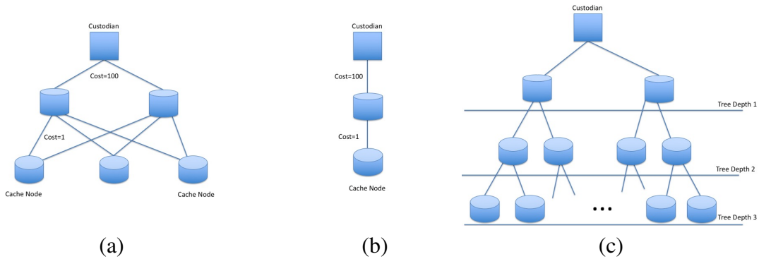
Figure 3. Hierarchical topologies: (a) layered; (b) chain and (c) tree.
